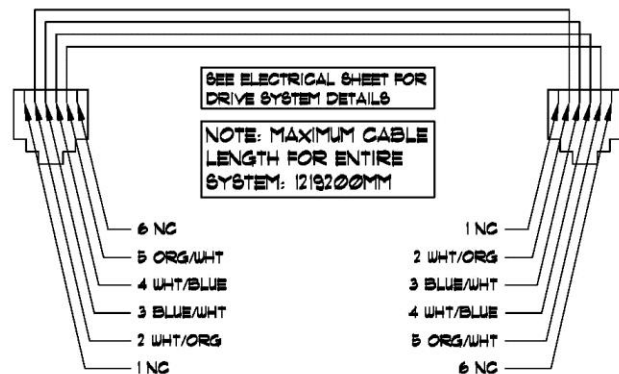
TYPICAL CONNECTION SCHEME
