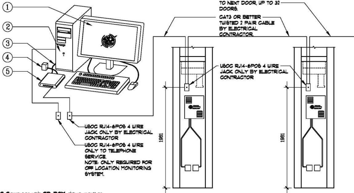
TYPICAL CONNECTION SCHEME
